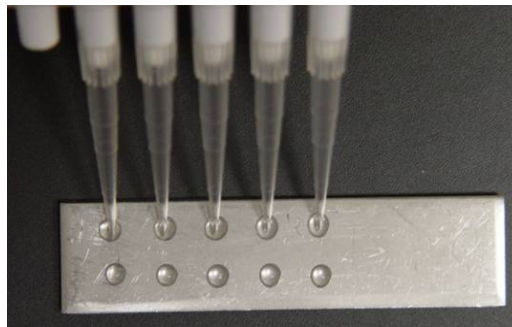
Figure 1. Liquid inoculation of coupon using a micropipette.
